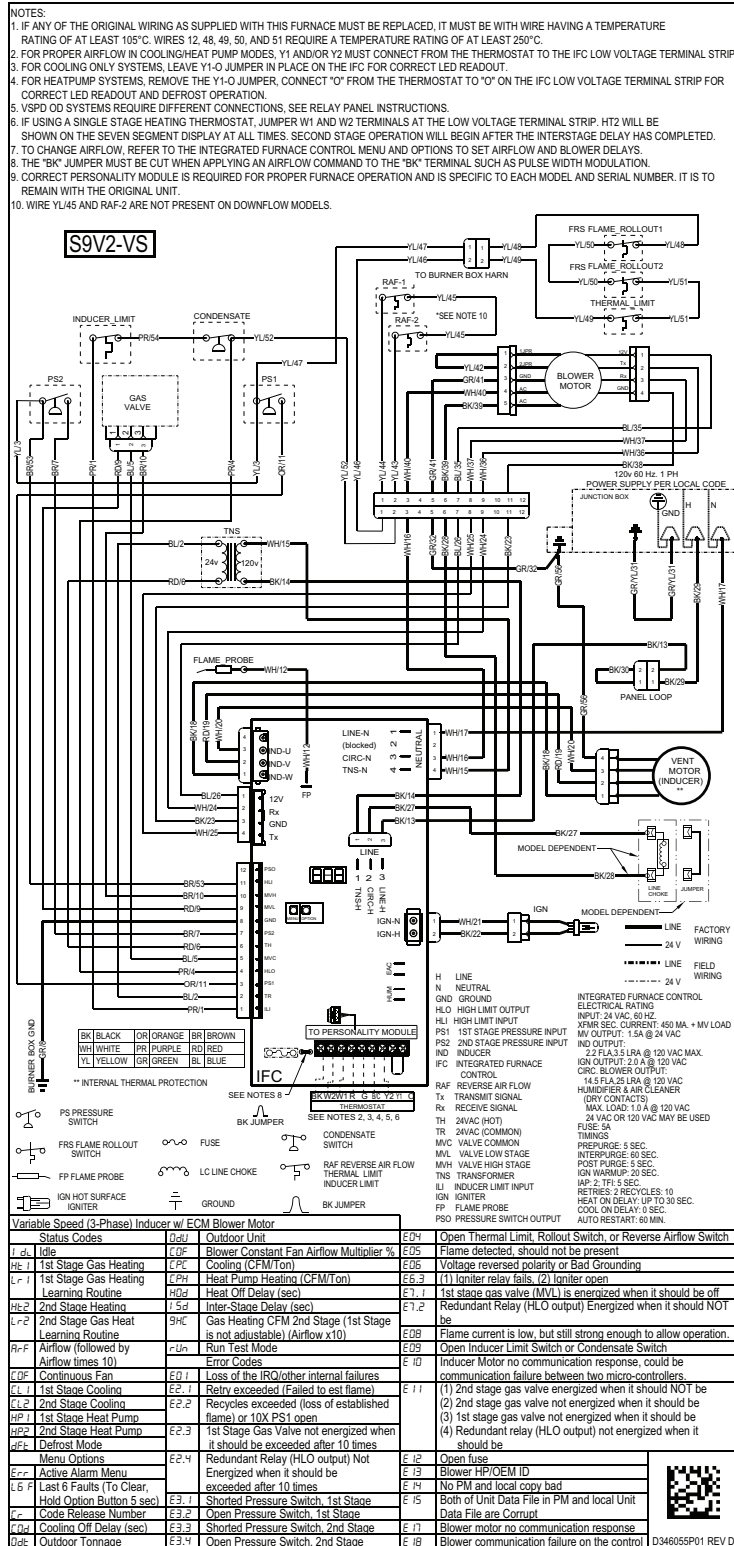
Figure 1. S9V2-VS wiring diagram
