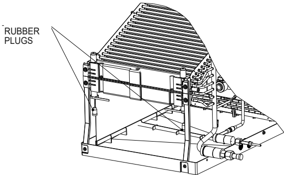
Completed Step. 14b View Horizontal Left Coil Assembly
