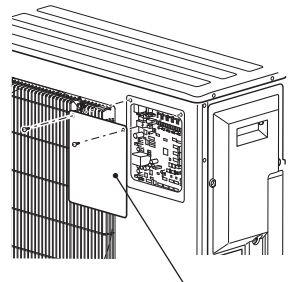
Maintenance panel
