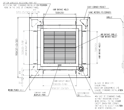
PLA-AENL ① ② A B C D E F 12~18 REFRIGERANT PIPE #2.5 (FLARE) CONNECTION 1/4" REFRIGERANT PIPE #2.7 (FLARE) CONNECTION 1/2" 241 79-1/20 250 C10-5/320 76 C2-62/64 76.5 C3-16/4 265/10-7/16 250/10-3/32 DR MORE DR LESS 24~40 REFRIGERANT PIPE #5.0 (FLARE) CONNECTION 3/8" REFRIGERANT PIPE #5.88 (FLARE) CONNECTION 5/8" 281 C1-1/16 291 C1-2/16 79.5 C1-1/8 79.5 C1-1/8 305/12 450/12-7/32 DR MORE DR LESS
