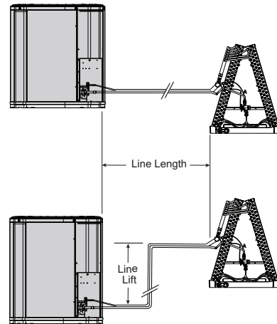
Figure 2. Line length
