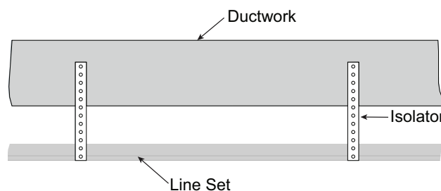
Figure 14. Incorrect lineset installation
