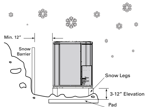
Figure 5. Cold climate considerations
