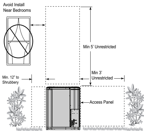
Figure 3. Location considerations
