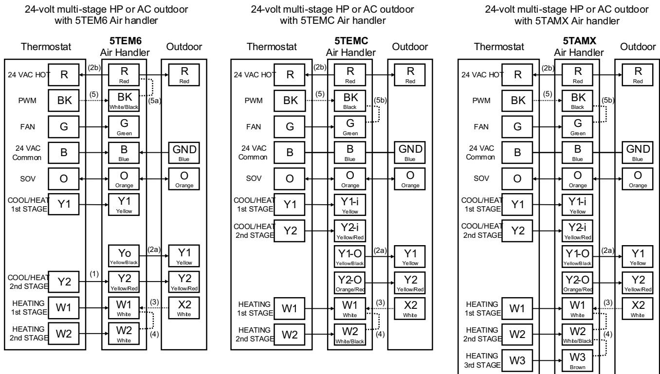
Figure 27. Connection diagrams – 5TEM6, 5TEMC, and 5TAMX
