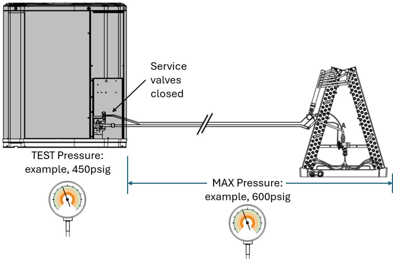
Figure 21. Check for leaks
