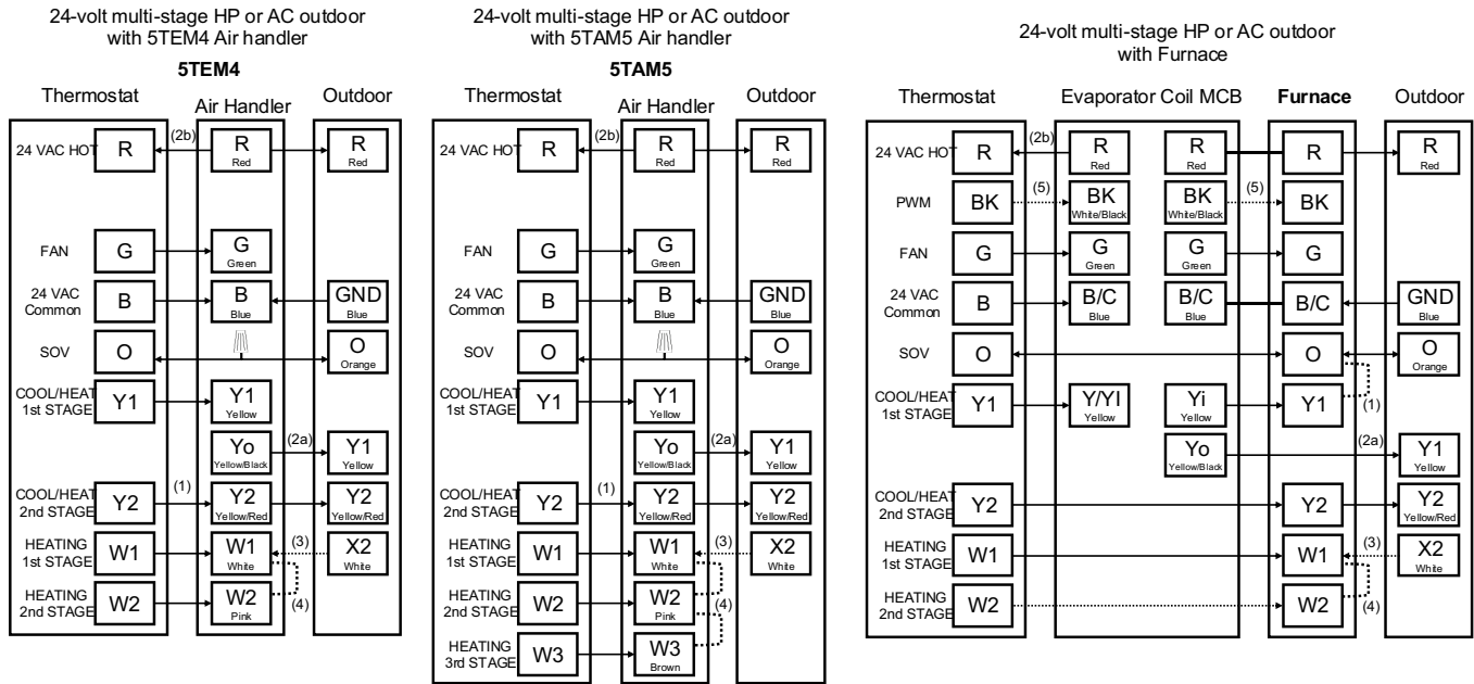
Figure 26. Connection diagrams – 5TEM4, 5TAM5
