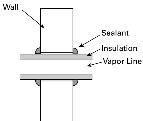
Figure 13. Isolation through the wall
