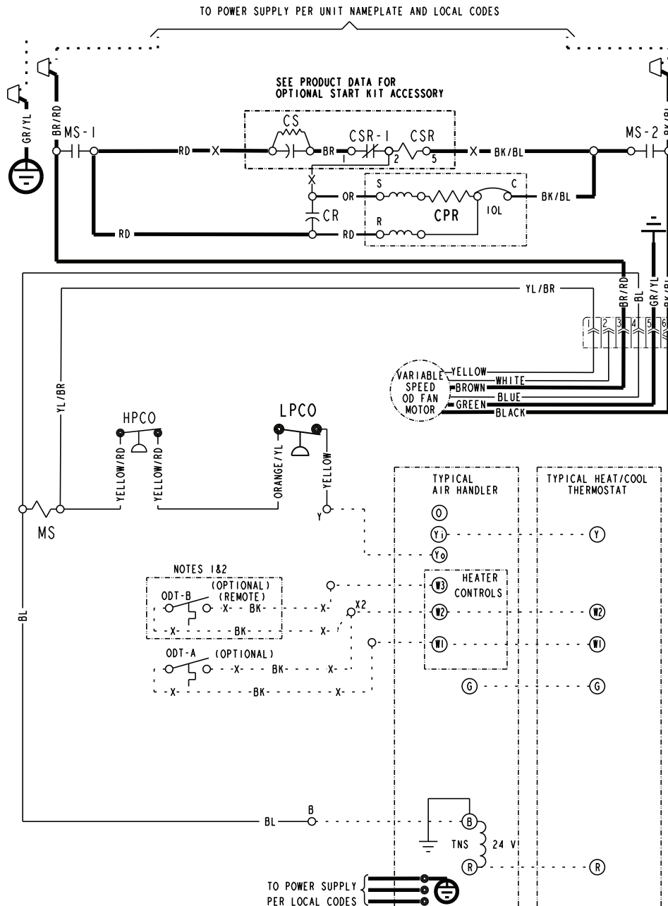
Figure 3. Model — 5TTX5060A
