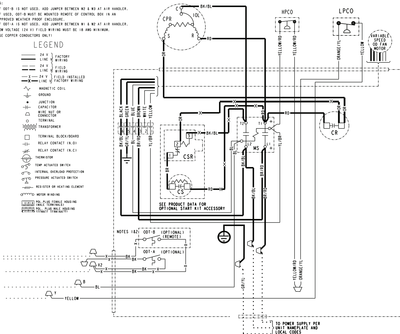
Figure 4. Model — 5TTR5060A
