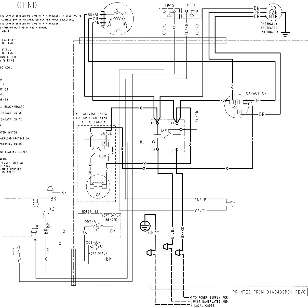
Figure 6. Model – 5TTR3060A
